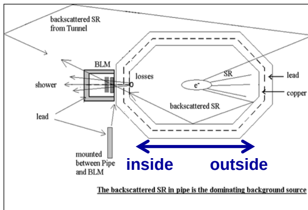
Fig. 2: The directions of synchrotron radiation and losses
