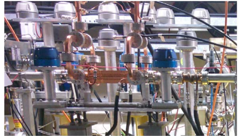
(a) The BLM (red fibre) above the CLIC structure (in the middle)
