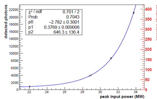
(a) Electron field emission
