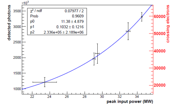
(b) RF breakdown
